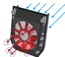
Reverse air-flow removes debris from radiator (cleaning cycle)
